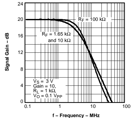
Figure 69. Signal Gain vs Frequency, V_S = 3\text{ V}
