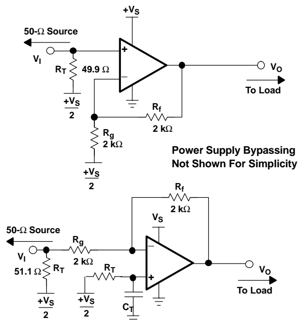
Figure 72. DC-Coupled Single Supply Operation
