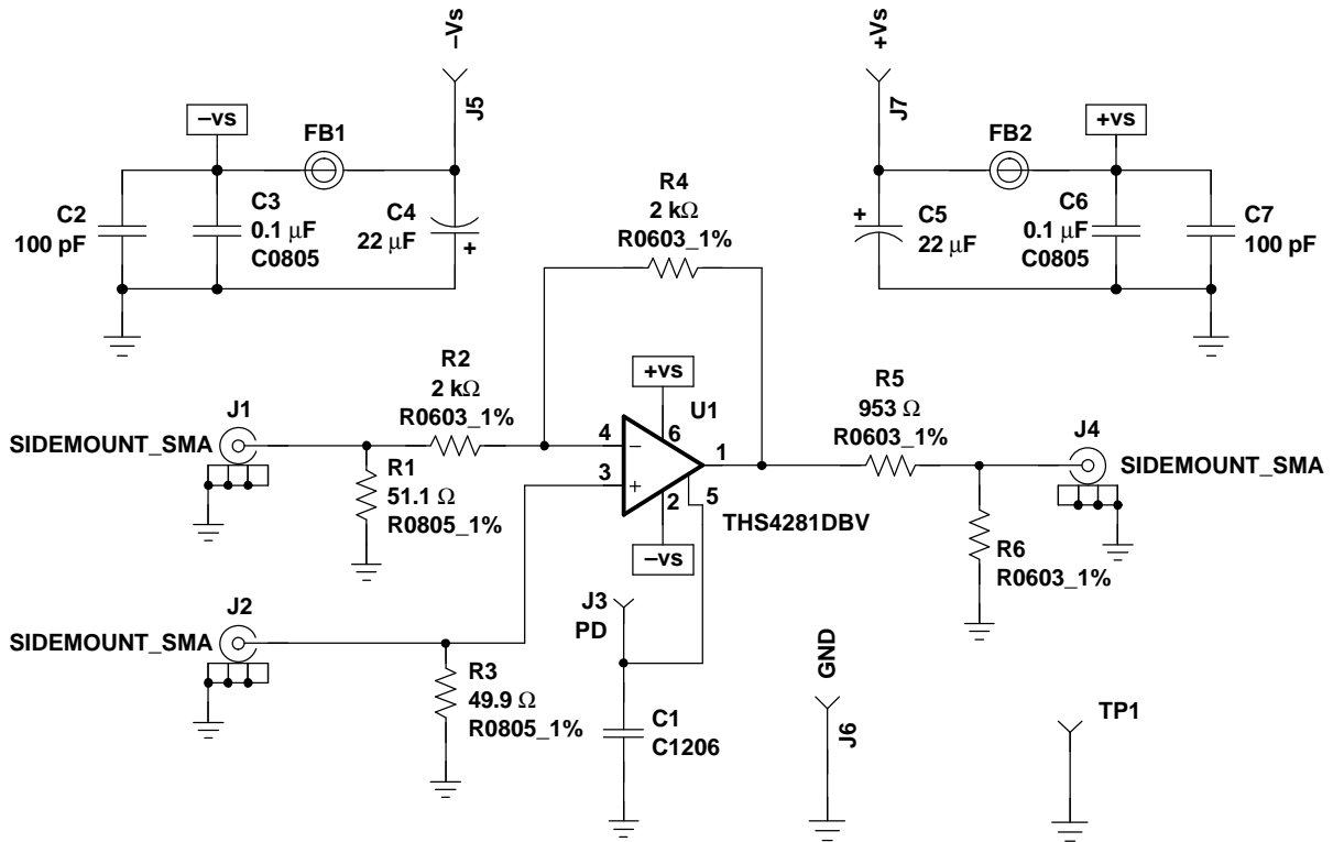
Figure 77. THS4281EVM Schematic
